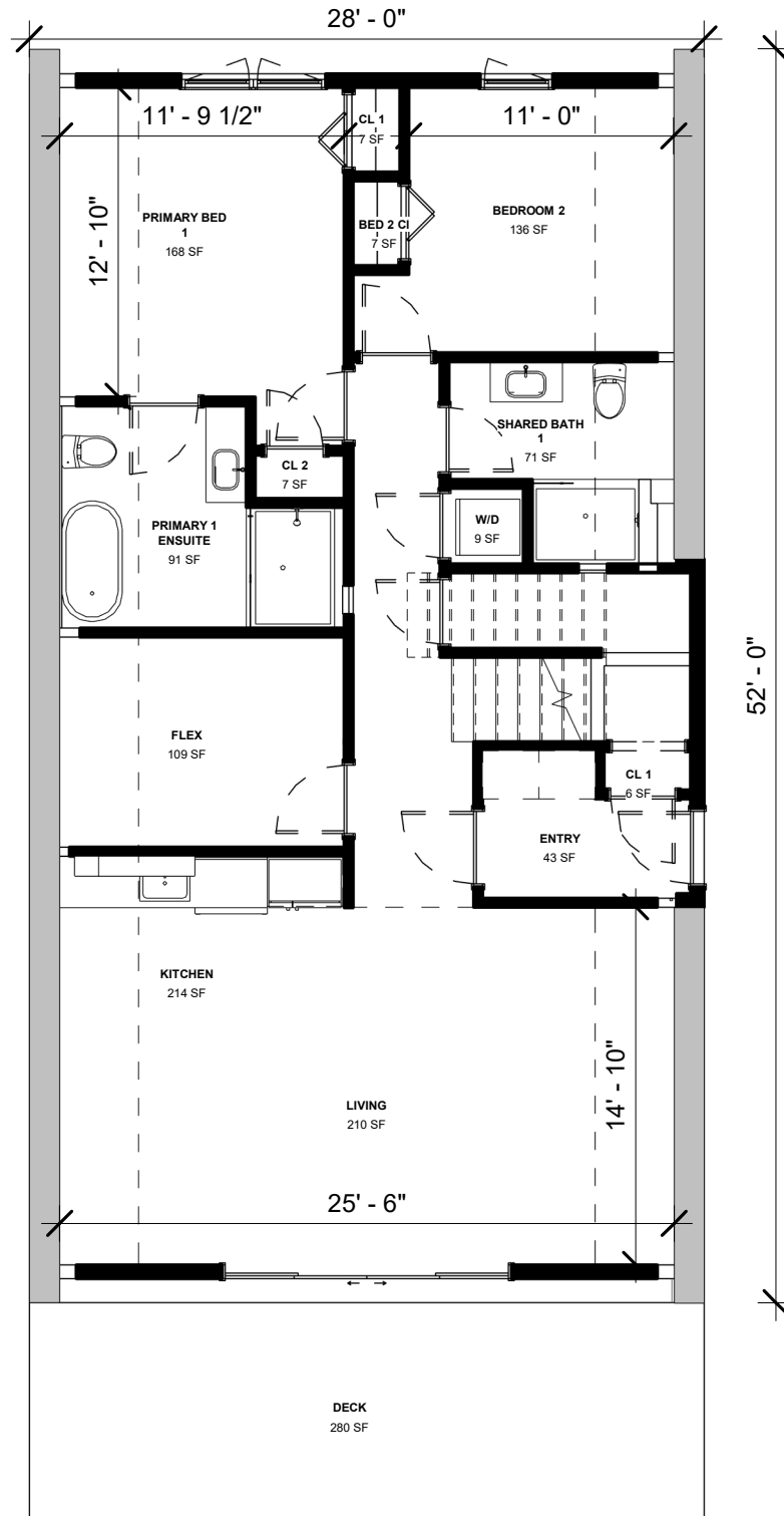
1 FIRST FLOOR - MARKETING PLAN 1/8" = 1'-0"
